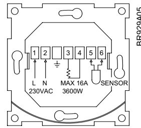
Connections
