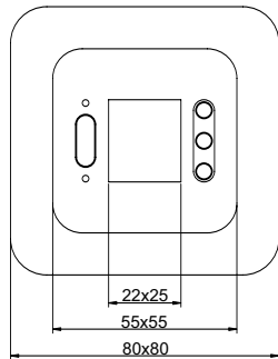
Dimensions (mm)
